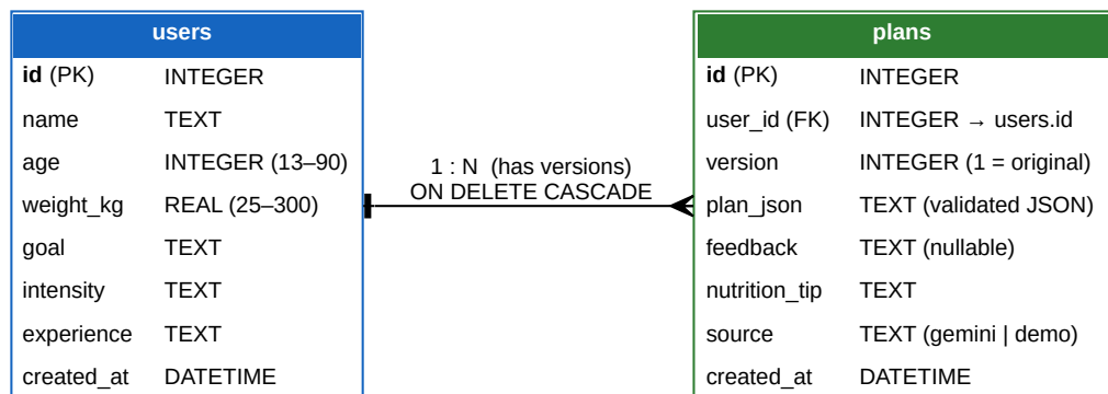
Figure 2: Entity-relationship diagram
